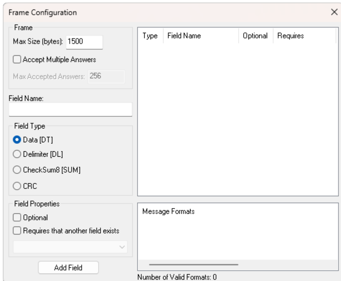
Janela Frame Configuration
