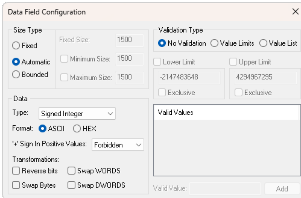
Janela Data Field Configuration
