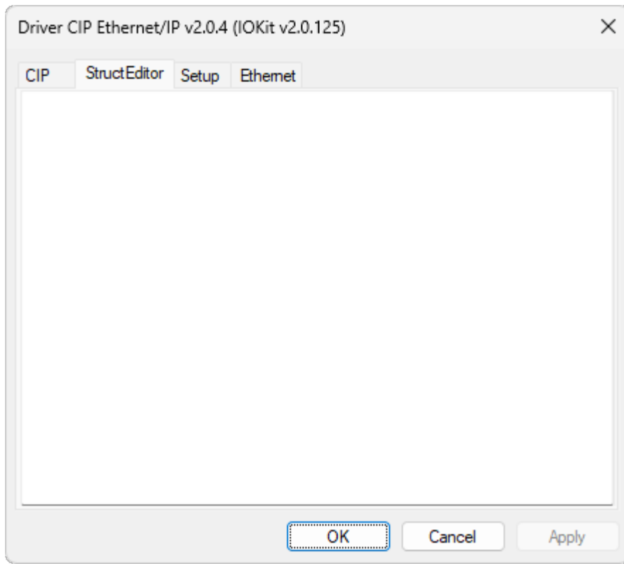
StructEditor tab
