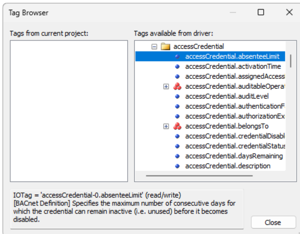
Generic BACnet Device node
