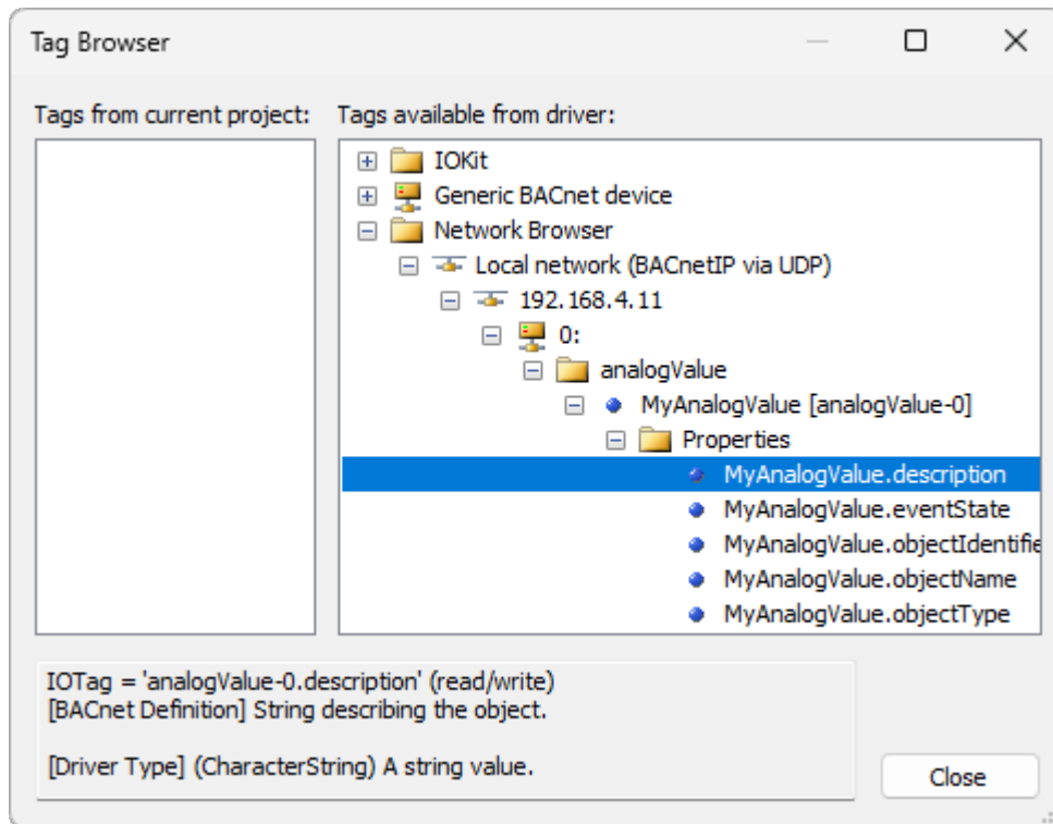
Network Browser node
